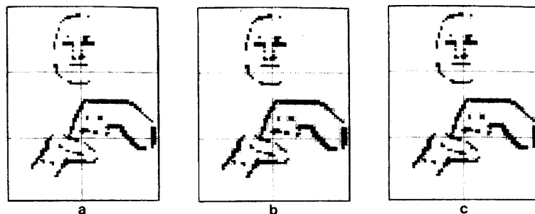
FIG. 13. The description of an ASL image by three different 2-dimensional hierarchical codes: (a) quadtree; (b) binary tree with horizontal dominance; (c) adaptive hierarchical code. (Cuts are shown in gray.)
