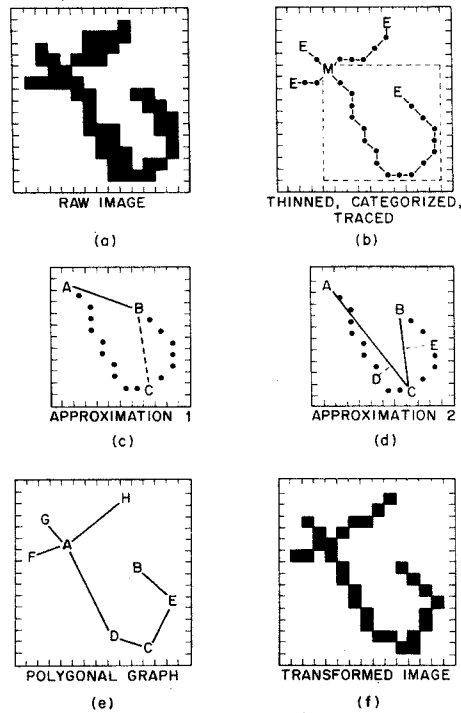
FIG. 9. Generating a polygonal transformation: (a) A portion of a cartoon generated by L96-5 (dark side Laplacian, 5% black), the input image. (b) After thinning, categorizing, and tracing. ( M ) is a multiple branch point , ( E ) is an endpoint . Panels (c) and (d) refer only to the subarea enclosed in dashes. (c) The first approximation ( A - B ) fails because point C is too far away. (d) The second approximation incorporates point C but fails because points D and E are too far. (e) The third approximation incorporates points D and E , and satisfies the distance criterion. (f) The polygonally transformed image derived from the polygonal graph (e).
