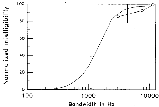
FIG. 17. Comparison of the bandwidth-intelligibility trade-off for acoustically coded speech and raster-coded ASL. The smooth ogival curve is taken from speech intelligibility data reported by French and Steinberg [78]. The three connected open circles represent ASL grey-scale data (OR96, OR48, OR24, all 15 fps) from Experiment 2. The vertical bars represent the performance of the middle 75% of subjects in Sperling's [11] ASL television experiment, assuming an effective frame rate of 15 fps.
