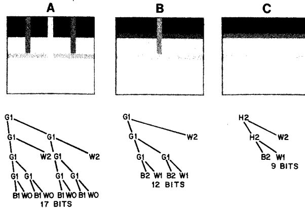
FIG. 12. A simple image (horizontal black bar) and its representation by three hierarchical codes, the level of grey indicates the level of cut: (a) binary tree code with vertical dominance, (b) binary tree code with horizontal dominance, (c) adaptive hierarchical code. The letters indicate the labeling of the subimage; the adjacent digit indicates the number of bits in the code for that letter.
