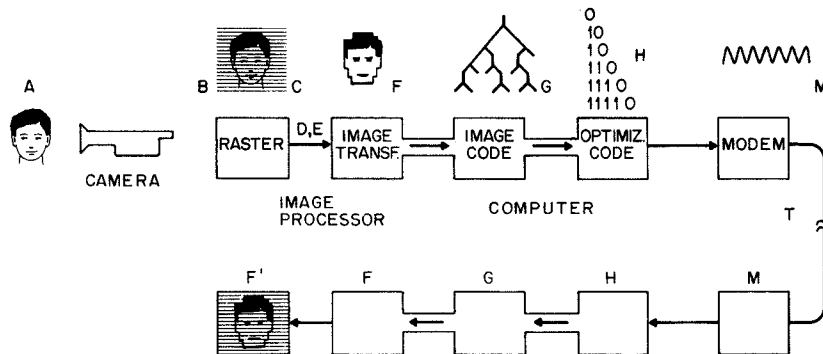
FIG. 3. Information transformations in a digital, low-bandwidth video communication system. Camera transforms optical array (A) into analog raster (B); image processor digitizes it (C) converting it into a computer-readable format (D); computer represents the image as an m \times n array in memory (E), and performs an image transformation (e.g., binary intensity-quantized image, F); the image is recoded (e.g., by a hierarchical code G which may span several images); this code may be further optimized (e.g., by a Huffman code, H); a modem converts the Huffmanized bit stream into a code (M) for transmission (T) through the switched telephone network. Decoding proceeds in reverse order up to the level of the transformed image (F) which is converted to raster representation (F') for viewing on a display monitor. In this scheme, information is lost between A and B but most critically in the transformation from E to F, hence no inverse transformation beyond F' is possible.
