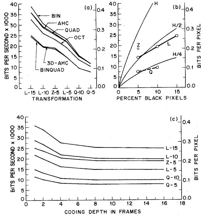
FIG. 15. The efficiency of image codes compared on representative ASL sequences: (a) The average code length in bits per second required to code six ASL image transformations, all at 15 fps. See Fig. 4 for key to transformations. The right-hand ordinates give the average bits per pixel (all images 96 \times 64 ). The curve parameter indicates the code (see text for details). Two-dimensional codes: (BIN) binary tree code; (AHC) adaptive hierarchical code; (QUAD) quadtree code; (OCT) oct-tree code; (3D-AHC) 3-dimensional adaptive hierarchical code; (BINQUAD) binquad code. (b) The efficiency of three optimally coded transformations ( Z , L , Q ) as a function of the percent of black or white pixels (whichever is smaller). For comparison, the theoretical minimum code length required to code a completely random picture with the same percent of black pixels (the information limit) is indicated by the curve H , showing that binquad-coded Q -transformed images use about H/4 , and L images about H/2 bits per pixel. (c) The efficiency of 3-dimensional binquad code as a function of the coding depth in frames for six ASL image transformations.
