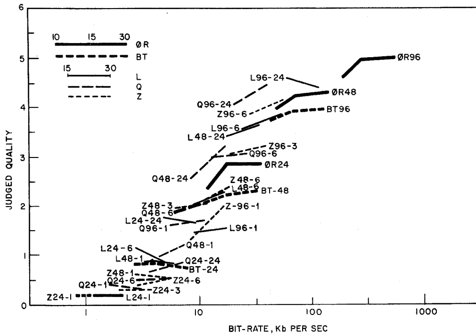
FIG. 6. Quality judgments as a function of bit rate for the 81 combinations of image transformations used in Experiment 1 and described in Table 2. In the curve labels, single letters (L, Q, Z) refer to binary images; double letters (OR, BT) to gray-scale images; see Fig. 4 for notation. The first number after the transformation code (96, 48, 24) refers to the vertical resolution in pixels; the number after the dash refers to the percent of black pixels in L and Z images, and to white pixels in Q images. Three frame rates (10, 15, 30 fps) are represented from left-to-right along the curves for gray-scale images; two rates (15, 30) for binary images. See Section 7 for details of the bit-rate computations.
