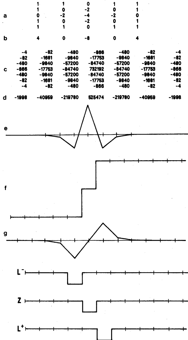
FIG. 5. Edge-detection convolution masks and their effects: (a) The 5 \times 5 mask used in Experiment 1 as a simple approximation to a Gaussian-smoothed Laplacian. The values in the rows and columns represent the values of the convolution operator at the corresponding x, y locations. (b) The projection of mask (a) onto the x axis—its response to a vertical line. (c) The 7 \times 7 mask used in Experiment 2 to better approximate a Gaussian-smoothed Laplacian (shown in opposite sign of (a)). Mask (c) is efficiently derived as a difference of Gaussians ( dog ) from separable 1-dimensional Gaussian masks. (d) Line response of (c). (e) Graphic representation of (d). (f) A steplike edge representing a 1-dimensional boundary. (g) Response of (c) to edge (f). (L - ) A pixel blackened at the minimum of (g), the dark side Laplacian transformation with black pixels at the dark side of edges. (Z) A pixel blackened at the zero crossing of (g), the zero-crossing transformation. (L + ) A pixel blackened at the maximum of (g).
