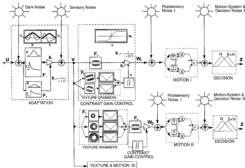
Fig. 11. Model of early visual processing. Suns, stationary-noise sources; rectangular boxes, linear filters; double rectangles enclose graphs of input–output relations. Triangles indicate gain-controlled amplifiers: the input (controlled signal) is the horizontal path; and the gain-controlling path is vertical. Adaptation. The visual input u passes through a separable space–time filter F_1 that in combination with the gain-control filter F_2 creates a receptive field of a given spatial scale (i.e., a visual channel). The gain of the amplifier k_1 is determined by the spatiotemporal surround \mu' of the through-signal. Amplifier gain is feedforward controlled by filters F_2 , which have greater spatial and greater temporal extents than those of controlled signal F_1 . For very small inputs, the gain-control signal u' is negligible and the receptive field is entirely positive (low pass) as indicated by the thick graphic plots in the double boxes. At high luminances, the receptive fields are bandpass, as indicated by the thin graphic plots. The orientation selectivity of first-order motion is represented by a spatial filter F_3 . Contrast-gain control of first-order motion is implemented as feedforward control by filters F_4 , which have a somewhat greater spatiotemporal extent ( \int f ) and cover a broader range of frequencies than the through-signal filter F_3 . The double boxes with a “V” inside indicate full-wave rectifiers whose outputs are approximately the absolute value of their inputs. Each combination of a filter and a rectifier is a texture grabber. The summed outputs of the texture grabbers determine gain control. In the second-order motion pathway, both the input and the gain control are created by summing the outputs of texture grabbers F_5 . The motion-controlling signal is summed over the surrounding area ( \int f ). The motion computation itself is similar to first-order (Motion I), which is represented here as a Reichardt detector. The decision process is represented as a maximum-likelihood decision between two alternatives (N, S+N). The third-order motion system is indicated only schematically by the rectangle (Motion III).
